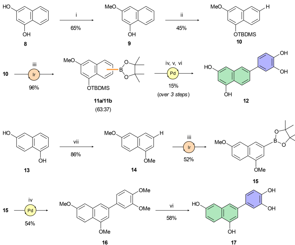
Scheme 2 Reagents and reaction conditions: (i) 4 M HCl (1,4-dioxane), MeOH, 0 °C → r.t., 24 h; (ii) TBDMSCl, imidazole, THF, 0 °C → r.t., 16 h; (iii) B_2(pin)_2 , [Ir(COD)OMe]_2 (4 mol%), bbbpy (6 mol%), n -hexane, 100 °C, 16–72 h; (iv) 4-bromoveratrole, SPhos Pd G2 (10 mol%), K_2CO_3 , THF/ H_2O (25:1), 100 °C, 16 h; (v) TBAF, THF, 0 °C, 2 h; (vi) BBr_3 , DCM, 0 °C → r.t., 2 h; (vii) MeI, K_2CO_3 , DMF, r.t., 18 h.
