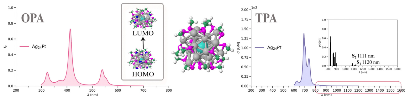
Fig. 3 TDDFT OPA (left) and TPA 71–73 (right) spectra calculated at the CAM-B3LYP 74 /def2-SVP 75 level of theory for \text{PtAg}_{24}(\text{SCH}_3)_{18} . For the Pt and Ag atoms the 19-electron relativistic effective core potential (19-e RECP) developed by the Stuttgart group 76 was implemented. DFT optimized structure with centrally doped single Pt atom is shown at the center, as well as HOMO–LUMO analysis. Atoms are colored by element: Ag in grey, Pt in turquoise, S in magenta, C in green, and H in white.
