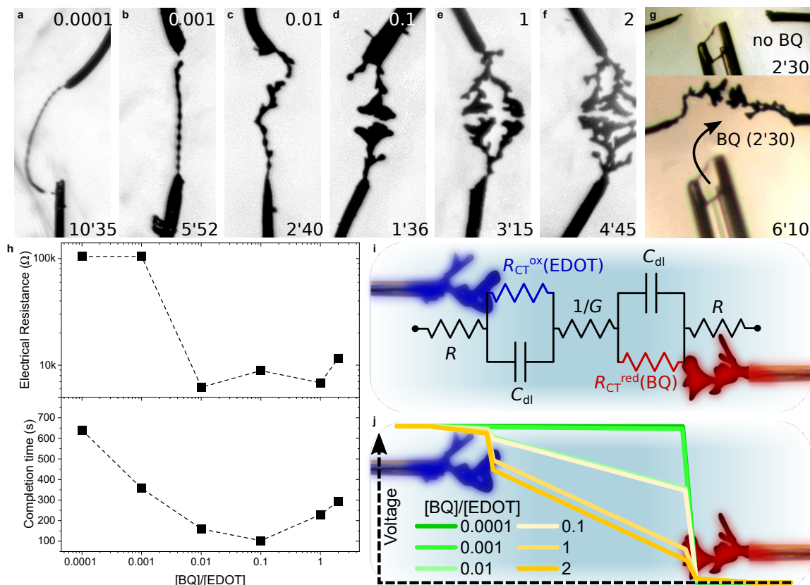
Figure 4: Influence of BQ as an Electroactive Counter-Agent CPD Morphogenesis in Water | a-f, Optical pictures of CPD growths (4 V p , 0 V off , 80 Hz, 50% dc , 10 mM [EDOT+BQ] and 1 mM NaPSS) in an aqueous medium with different [BQ]/[EDOT] molar ratios (values displayed at the top of each picture). Each image was taken a few seconds before CPDs merged (applied-voltage duration displayed at the bottom of each picture). g, Introduction of a BQ aqueous solution, triggering CPD growth in an aqueous solution containing 10 mM EDOT and 1 mM NaPSS. h, Dependence of the electrical resistance (through each CPD displayed in Fig. 4.a-f after they merged) and their growth duration on the [BQ]/[EDOT] molar ratio contained in the growth media. i, 7-Element equivalent circuit highlighting the contributions of [EDOT] and [BQ] on the charge-transfer balance between oxidation and reduction. j, Simulated voltage drop according to the equivalent circuit presented in Fig. 4.i, with R defined as half the experimental value of the CPD electrical resistance once merged, 1/G = 60 kΩ, R CT ox = 100 kΩ/mM EDOT and R CT red = 100 kΩ/mM BQ . Blue indicates the point of highest potential in the circuit, whereas red indicates the point of lowest potential.
