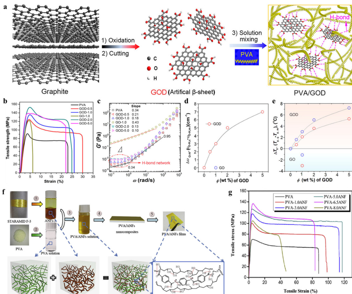
Fig. 6 (a) Diagram showing the synthesis of GOD and the process for fabricating PVA/GOD nanocomposites. (b) Tensile curves of PVA and PVA/GOD. (c) Frequency dependence of G' for PVA and PVA/GOD. (d) Wavenumber shift ( \Delta\nu_{O-H} ) and (e) T_g difference ( \Delta T_g ) of PVA and PVA/GOD compared to PVA. (a–e) Reproduced with permission. 31 © 2018 American Chemical Society. (f) Illustration of interactions between PVA and aramid nanofibers (ANFs). (g) Stress–strain curves of PVA and PVA/ANFs. (f and g) Reproduced with permission. 82 © 2017 Elsevier Ltd. All rights reserved.
