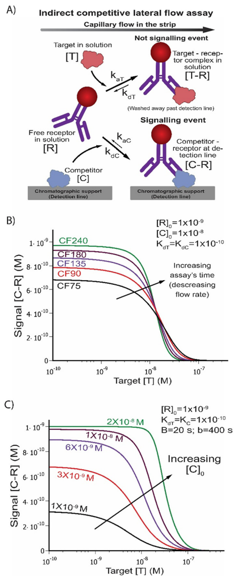
Fig. 5 Modelling of an indirect competitive assay using an analytical expression reported by Sotnikov and co-workers. 41 (A) Scheme of reactions involved in the indirect competitive LFA using a labelled antibody R in solution as a conjugate and the competitor immobilized on the detection line C . k_{aT} and k_{aC} are the kinetic association constants for T and C respectively, and k_{dT} and k_{dC} are the kinetic dissociation constants for T and C . (B) Implication of the capillary flow (CF) from detection pads of different porosity: higher porosity substrates (CF75, faster assay) and lower porosity (CF240, slower assay). Panel (C) displays the effects of different [C] in the detection line. B stands for the migration time from sample addition until the detection line, b is the total duration of the assay starting.
