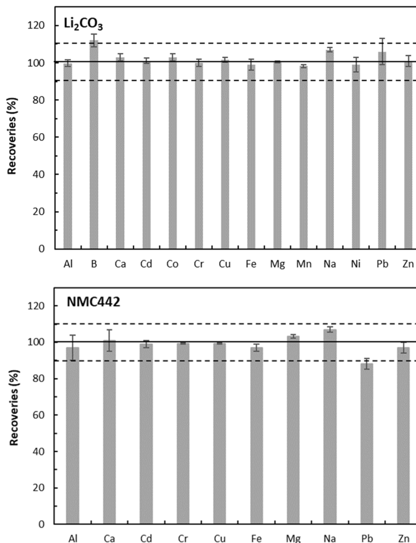
Fig. 3 Recoveries expressed as % (mean \pm SD, n = 3 ) obtained for the \text{Li}_2\text{CO}_3 raw material and NMC442 cathode analysed by MICAP OES. Q_g 0.9 \text{L min}^{-1} , Q_l 0.5 \text{mL min}^{-1} , TExposure: 1000 ms.
