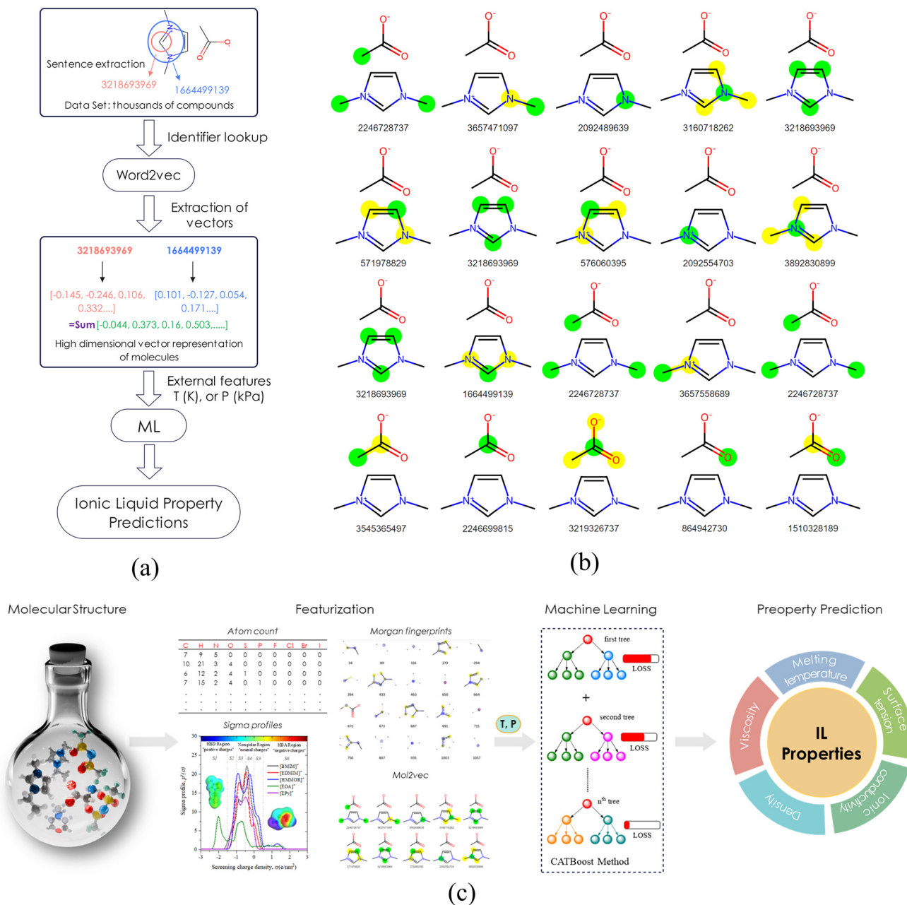
Fig. 1 (a) Overview of the generation and usage steps of Mol2vec. Mol2vec embeddings (i.e., vector representations of substructures) are generated via an unsupervised pretraining. (b) Depiction of identifiers obtained with the Morgan algorithm on the structure of 1,3-dimethylimidazolium acetate forming a molecular sentence. If an atom has more than one identifier, the first identifier for that atom is the one for radius 0, followed by radius 1, etc. (c) Schematic overview of machine learning framework for predicting multiphysical properties based on different input featurization techniques.
