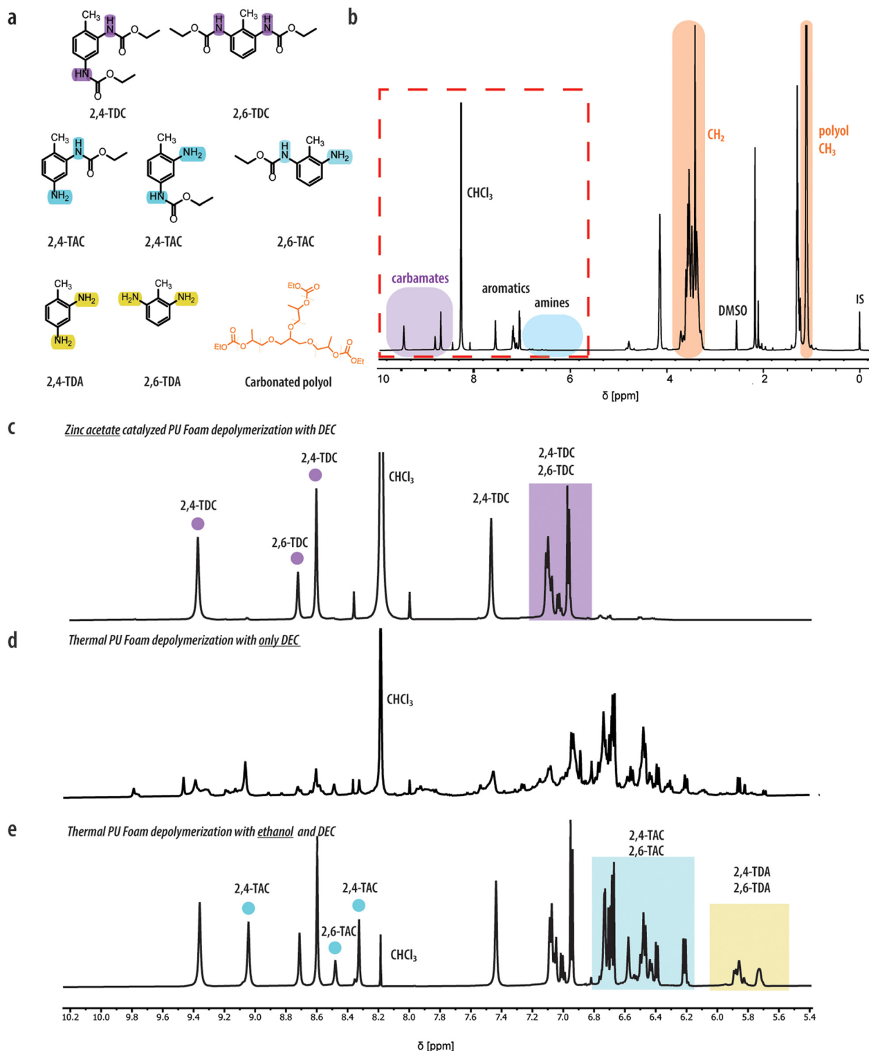
Fig. 2 Characterization of the liquid phase after PU depolymerization: (a) PUF depolymerization products. 1 H NMR spectra (recorded in 1 : 4 (v/v) CDCl 3 : DMSO- d 6 mixture) of the filtrate after separation of the solid fraction: (b) in a typical experiment with 0.4 g foam, 20 mL DEC and 20 mg Zn (OAc) 2 , without ethanol; (c) partial spectrum of B focusing on the aromatic region; (d) same region for the thermal, uncatalyzed PUF depolymerization with only DEC (0.4 g foam and 20 mL DEC); (e) same region for the PUF depolymerization with the cosolvent ethanol (0.2 g of foam, 4 : 6 ethanol : DEC ratio with a total of 10 mL), without Zn(OAc) 2 .
