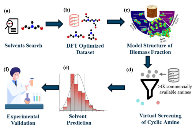
Fig. 1 Workflow of the proposed methodology. (a) Data were collected from the literature on amines used as solvents; (b) the COSMO-RS model was applied to a diverse dataset containing 650 cyclic amine structures by first optimizing and generating the cosmo file; (c) the model structure of different biomass fractions; mainly cellulose, hemicellulose, and lignin were generated; (d) the activity coefficients of different biomass fractions were calculated for the different cyclic amines; (e) solvents were ranked based on the solute-solvent activity coefficient; and (f) solvents predicted to be the most effective were selected for further study and experimental testing.
