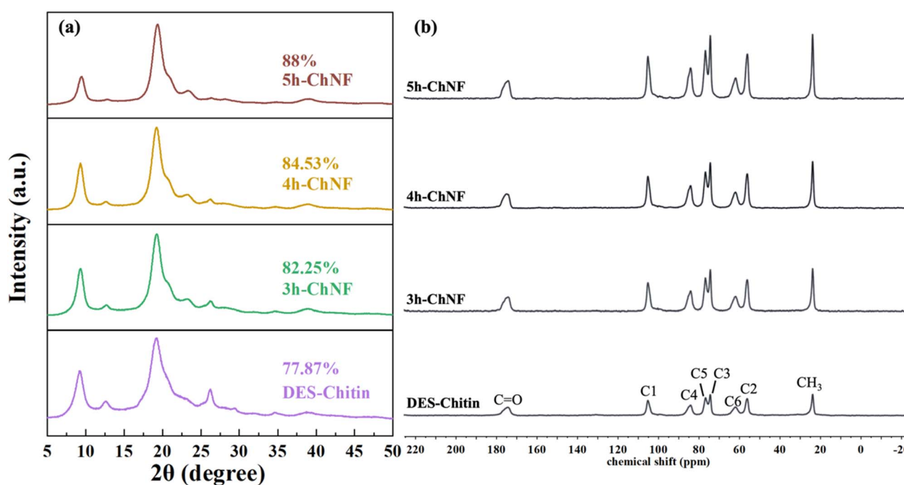
Fig. 2 (a) XRD spectra of DES-Chitin, 3h-ChNF, 4h-ChNF, and 5h-ChNF, with their respective crystallinity index shown above each spectrum; (b) ^{13}C solid-state NMR spectra of DES-Chitin, 3h-ChNF, 4h-ChNF, and 5h-ChNF.
