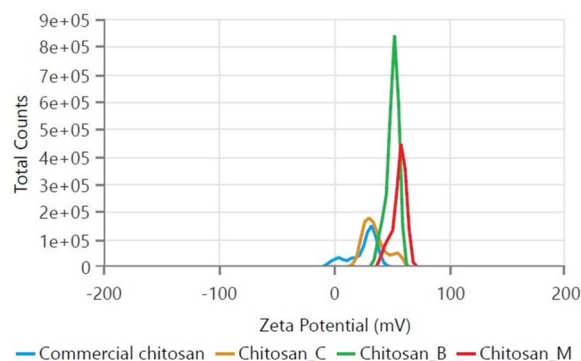
Fig. 2 Zeta potential (mV) of chitosan that was commercially purchased or generated from the crickets from chitin isolated through the chemical (Chitosan_C), biological (Chitosan_B) and microwave-assisted method (Chitosan_M).
