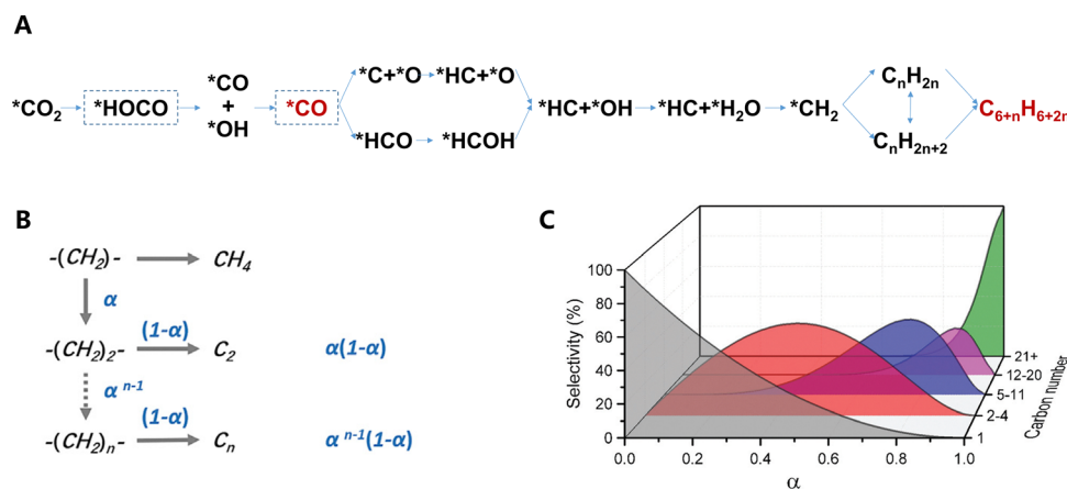
Fig. 11 (A) Reaction pathways for CO 2 -to-aromatics via the modified Fischer–Tropsch synthesis route. (B) Chain-growth probability \alpha . (C) Regulating the carbon chain length distribution of products by chain-growth probability \alpha . Reprinted and reproduced with permission from Wang et al. Copyright (2021), Elsevier Inc., 4 and Zhou et al. Copyright (2019), The Royal Society of Chemistry. 80
