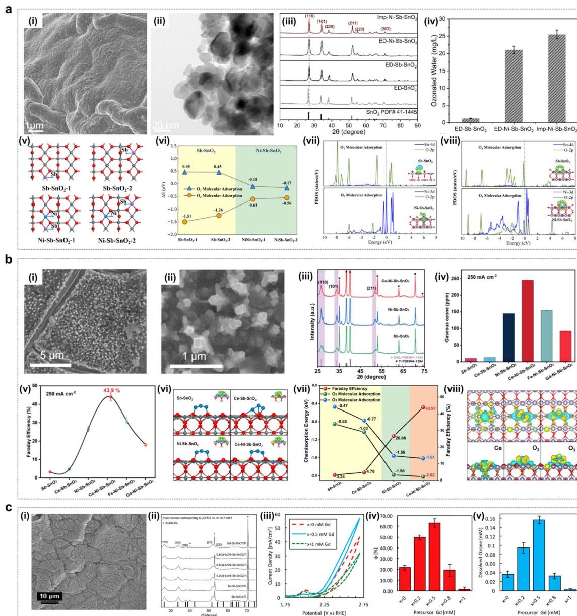
Fig. 11 Doped \text{SnO}_2 catalysts for the EOP process. (a) (i) and (ii) SEM and HRTEM images of \text{Imp-Ni-Sb-SnO}_2 , \text{ED-Ni-Sb-SnO}_2 , \text{ED-Sb-SnO}_2 , and \text{ED-SnO}_2 electrocatalysts. (iii) and (iv) XRD patterns and the ozonated water concentration of \text{Imp-Ni-Sb-SnO}_2 , \text{ED-Ni-Sb-SnO}_2 , \text{ED-Sb-SnO}_2 , and \text{ED-SnO}_2 electrocatalysts. (v) and (vi) DFT-calculated structure and adsorption energy of \text{Sb-SnO}_2 -1, \text{Sb-SnO}_2 -2, \text{Ni-Sb-SnO}_2 -1, and \text{Ni-Sb-SnO}_2 -2. (vii) and (viii) Projected density of states (PDOS) and charge density differences for \text{O}_2 (vii) and \text{O}_3 (viii) adsorption on \text{Sb-SnO}_2 and \text{Ni-Sb-SnO}_2 surfaces. (Reprinted with permission from ref. 52. Copyright John Wiley and Sons 2024.) (b) (i) and (ii) SEM images of \text{Ce-Ni-Sb-SnO}_2 . (iii) XRD spectra of \text{Ce-Ni-Sb-SnO}_2 , \text{Ni-Sb-SnO}_2 , and \text{Sb-SnO}_2 . (iv) and (v) Gaseous ozone production and faradaic efficiency of the series of electrocatalysts. (vi) Geometric structures and charge density differences of \text{O}_3 adsorbed on \text{Sb-SnO}_2 , \text{Ce-Sb-SnO}_2 , \text{Ni-Sb-SnO}_2 , and \text{Ce-Ni-Sb-SnO}_2 . (vii) Relationship between chemisorption energy of \text{O}_2 and \text{O}_3 and faradaic efficiency on the four surfaces. (viii) Charge density differences associated with Ce doping on \text{Ce-Ni-Sb-SnO}_2 ; \text{O}_2 , and \text{O}_3 adsorption on \text{Ce-Ni-Sb-SnO}_2 . (Reprinted with permission from ref. 53. Copyright Wiley 2023.) (c) (i) SEM image of the EOP electrocatalyst exhibiting a typical "cracked mud" morphology. (ii) XRD patterns of synthesized electrocatalyst thin films showing the cassiterite \text{SnO}_2 bulk structure for all dopants. (iii) Representative cyclic voltammetry (CV) curves for Ni-only ( x = 0 ), Gd-only ( x = 1 ), and Ni-Gd ( x = 0.5 ) samples. (iv) and (v) Faradaic efficiency of ozone production and concentration of dissolved ozone measured after 60 seconds at 2.7 V vs. RHE. (Reprinted with permission from ref. 65. Copyright John Wiley and Sons 2021.)
