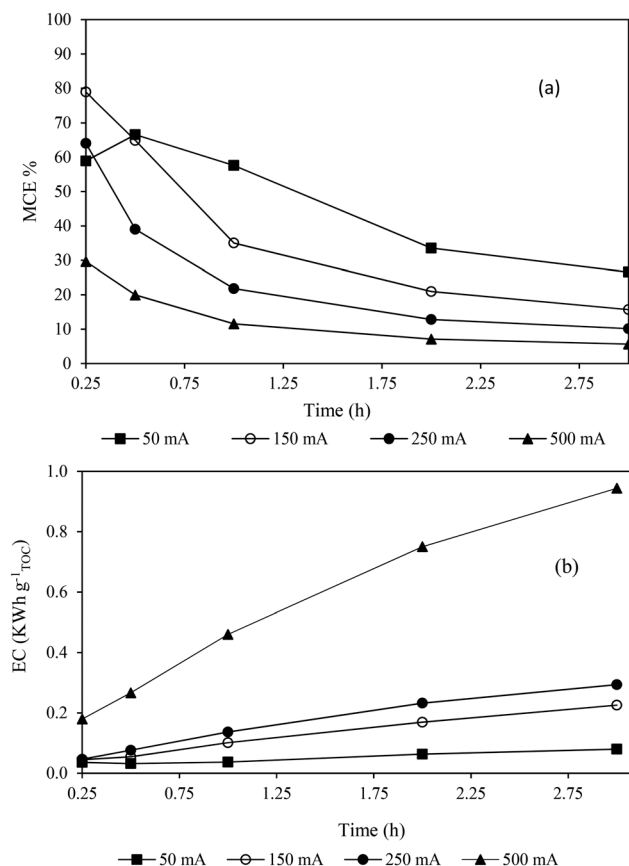
Fig. 3 Mineralization current efficiency (% MCE) (a) and energy consumption ( EC_{TOC} ) (b) as a function of electrolysis time of 50 mg L -1 of miconazole corresponding to 25.95 mg L -1 initial TOC by electro-Fenton under operating conditions of [Na_2SO_4] = 50 mM, Fe^{2+} = 0.2 mM and pH = 3.0.
