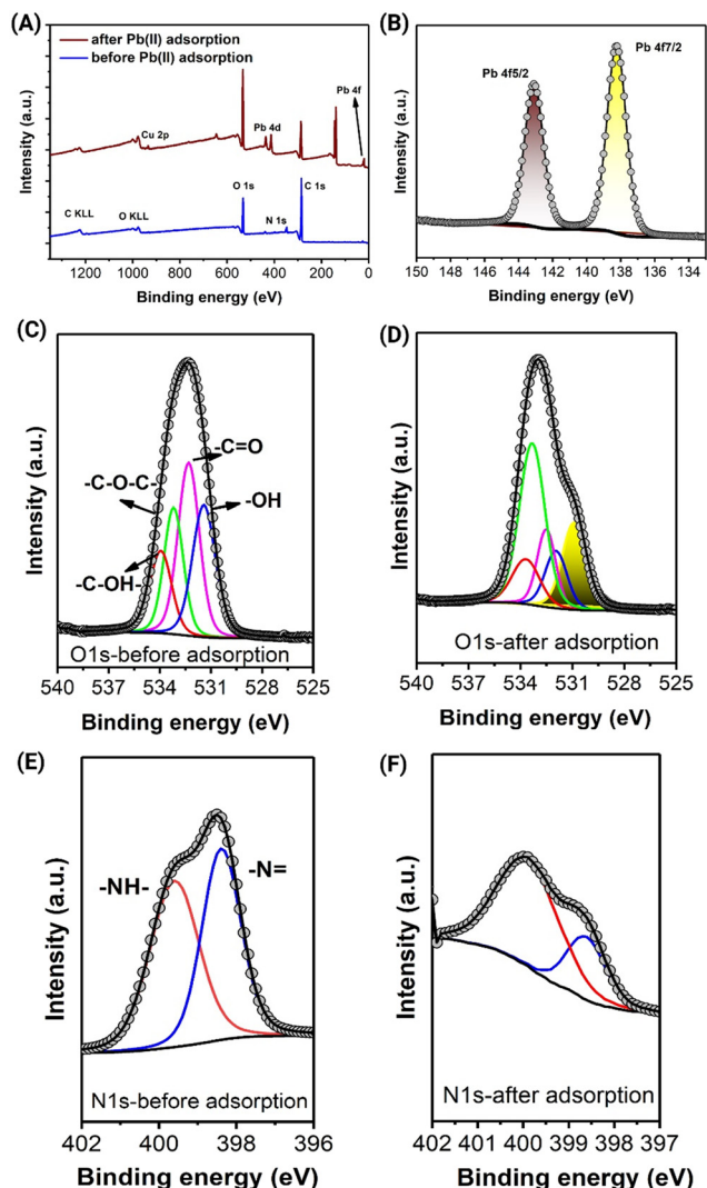
Fig. 6 (A) XPS survey spectra of CA-BNMG-1 beads before and after Pb(II) adsorption. (B–F) High-resolution spectra with deconvolution: (B) Pb 4f after adsorption, (C) O 1s before adsorption, (D) O 1s after adsorption, (E) N 1s before adsorption, and (F) N 1s after adsorption.
