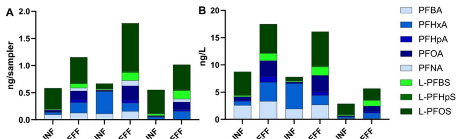
Fig. 5 Target PFAS detected in mPEs (A), and estimated time-weighted average water concentrations derived from mPE concentrations based on estimated passive sampling rates (B).
