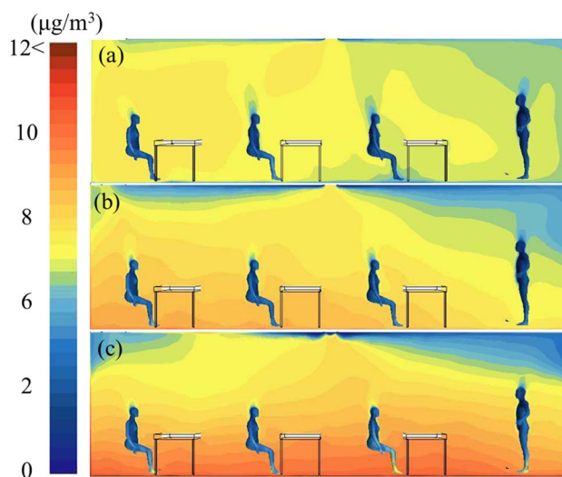
Fig. 6 Distribution of SOA concentrations under mixing ventilation with an inlet air temperature of (a) 14 \text{ }^{\circ}\text{C} (case 4, cooling), (b) 38 \text{ }^{\circ}\text{C} (case 5, heating), (c) 50 \text{ }^{\circ}\text{C} (case 6, heating).
