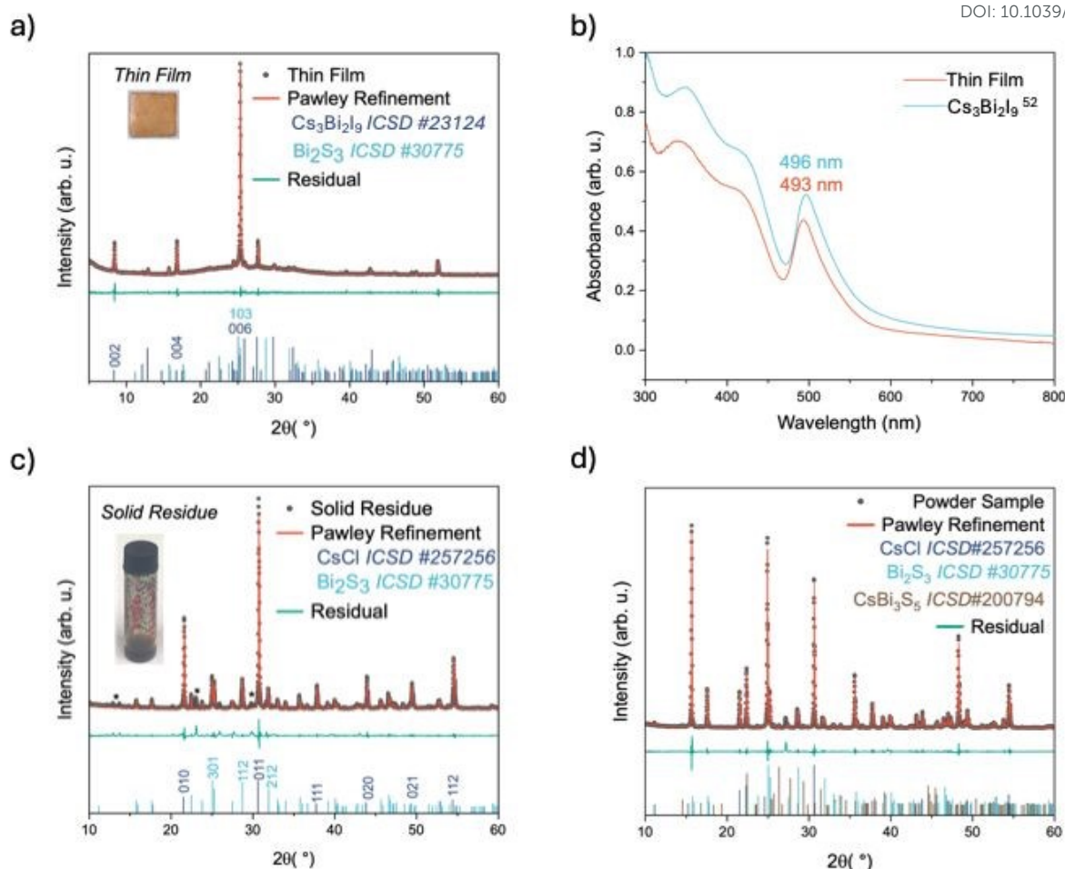
Figure 3. Challenges with \text{CsBiSbCl}_2 synthesis (a) PXRD pattern of thin films synthesized according to Huang et al. (solid circles), with the corresponding Pawley refinement to \text{Cs}_3\text{Bi}_2\text{I}_9 and \text{Bi}_2\text{S}_3 (red line); R_{wp} = 9.1874 GoF = 1.2124. Inset: Photograph of the as-prepared thin film on 1.4 cm 2 glass. (b) UV-Vis absorption spectrum of prepared thin films and \text{Cs}_3\text{Bi}_2\text{I}_9 reference spectrum, 52 with the characteristic \text{Cs}_3\text{Bi}_2\text{I}_9 excitonic peaks labelled. (c) PXRD pattern of solid residue from precursor solution from the attempted synthesis of \text{CsBiSbCl}_2 (solid circles), with the corresponding Pawley refinement to \text{Bi}_2\text{S}_3 and \text{CsCl} (red line); R_{wp} = 12.9970 GoF = 2.1417, unidentified peaks are labelled by *. Inset: Photograph of the solid residue in a glass vial. (d) PXRD pattern of material from attempted solid-state synthesis of \text{CsBiSbCl}_2 (solid circles), with the corresponding Pawley refinement to \text{CsCl} , \text{Bi}_2\text{S}_3 , and \text{CsBi}_3\text{S}_5 (red line); R_{wp} = 10.9693 , GoF = 1.7417.
