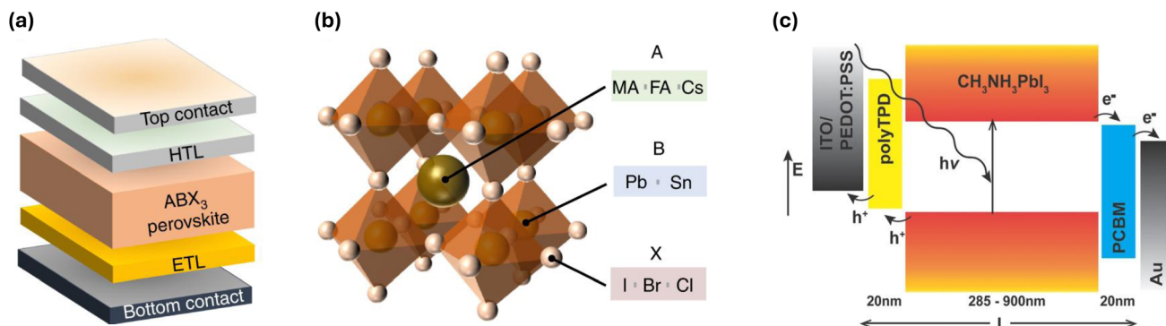
Fig. 1 (a) Typical perovskite solar cell structure. (b) \text{ABX}_3 crystal structure of perovskite absorbers. MA, FA and Cs stand for methylammonium, formamidinium, and cesium, respectively. (c) Energy level diagram of a PSC consisting of ITO as TCO, PolyTPD as the HTL, \text{CH}_3\text{NH}_3\text{PbI}_3 as the absorber, PCBM as the ETL and gold (Au) as the top contact metal electrode. (a) and (b) are adapted with permission from ref. 5, copyright ©2022, Springer Nature. (c) is adapted with permission from ref. 6, copyright 2017, John Wiley and Sons.
