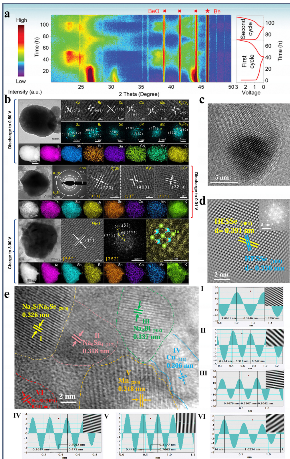
Fig. 4 (a) In situ XRD along with the GCD profiles of InGeSiP 3 . Reproduced with permission. 47 Copyright 2024, Wiley-VCH. (b) TEM image, IFFT patterns, and SAED pattern of Sb 1.4 Bi 0.2 Sn 0.2 Co 0.1 Mn 0.1 Te 3 when charging and discharging. Reproduced with permission. 44 Copyright 2025, American Chemical Society. (c)–(e) HRTEM images for the Cu 0.88 Sn 0.02 Sb 0.02 Bi 0.02 Mn 0.02 S 0.9 Se 0.1 electrode at 0.1 V and (I–VI) corresponding intensity profiles and fast Fourier transform (FFT) pattern; HRTEM images of Sn 3.0 V states and corresponding FFT patterns. Reproduced with permission. 49 Copyright 2025, Nature Publishing Group.
