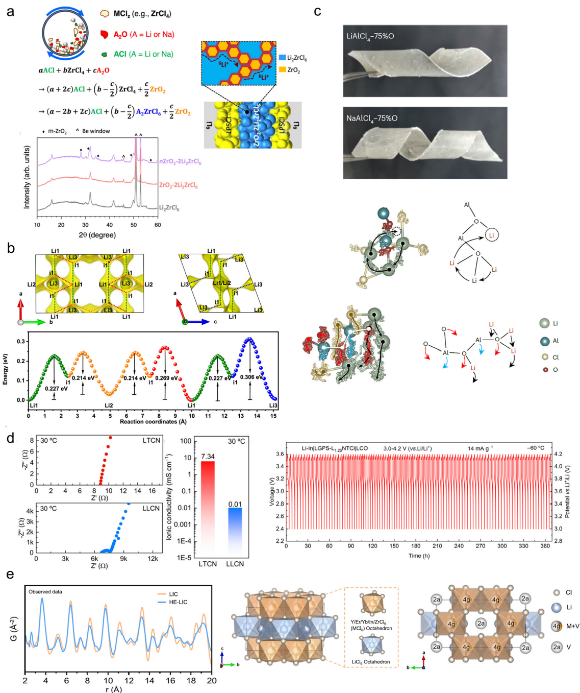
Fig. 5 (a) Preparation of \text{ZrO}_2(\text{-ACl})\text{-A}_2\text{ZrCl}_6 ( \text{A} = \text{Li} or \text{Na} ) through a two-step ball-milling synthesis method, and the schematic diagram of the interfacial superionic \text{Li}^+ diffusion pathways. 101 (b) \text{Li}^+ migration pathways and migration energy barriers in \text{Li}_3\text{Zr}_{0.75}\text{OCl}_4 . 102 (c) The hopping and migration of \text{Li}^+ in the viscoelastic electrolytes LACO and NACO. 39 (d) The high ionic conductivity and excellent extremely low temperature performance of amorphous nitrogen-halide electrolytes \text{Li}_{3x}\text{TaCl}_5\text{N}_x . 105,106 (e) The local structure and unit cell of HE-LiC. 107
