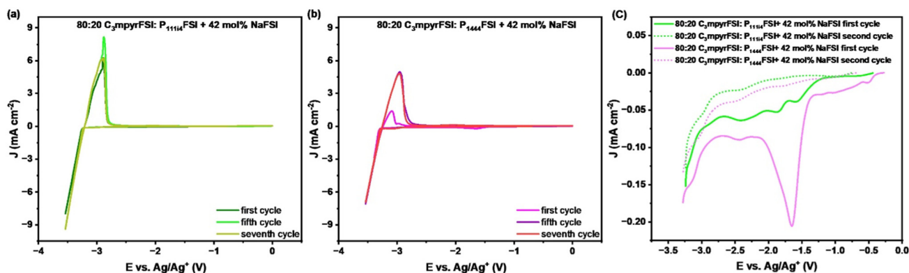
Fig. 3 Three-electrode cyclic voltammetry curves for mixed ILs. (a) C_3\text{mpyrFSI}/P_{1114}\text{FSI} mixture, (b) C_3\text{mpyrFSI}/P_{1444}\text{FSI} mixture, (c) enlarged view of the first and second cycles prior to the onset of Na deposition.
