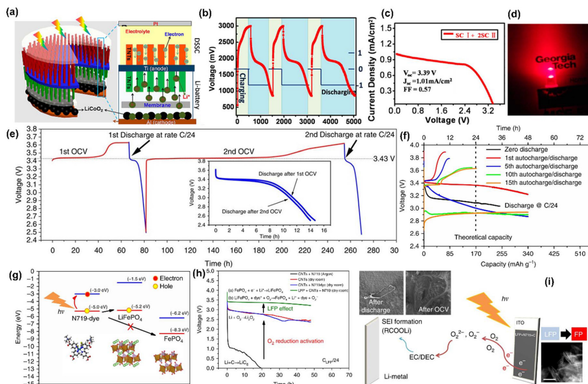
Fig. 9 (a) Design and principle of an integrated DSSC and Li-ion battery with \text{TiO}_2 nanotubes, (b) discharge/charge cycling performances, (c) J - V curves of the DSSC with three tandem cells (SC I and 2SC II) connected in series, (d) LED powered by using the storage energy. 45 Copyright: 2012 American Chemical Society. (e) V_{\text{OC}} and (f) GCD curves of \text{LiFePO}_4 , (g) energy band alignment of the photocathode components, (h) discharge curves of films in different gas atmospheres at C/24 discharge rate, (i) photoassisted charging mechanism of LFP(dye)/electrolyte/Li cell. 7 Copyright: 2017 Nature.
