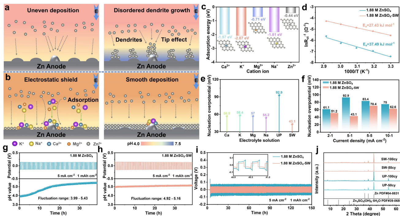
Fig. 1 Schematic illustration of zinc deposition in (a) \text{ZnSO}_4 and (b) \text{ZnSO}_4 -seawater electrolytes; (c) adsorption energy of \text{Na}^+ , \text{K}^+ , \text{Ca}^{2+} , \text{Mg}^{2+} , and \text{Zn}^{2+} ions on the surface of the zinc metal; (d) interfacial activation energy barrier of \text{Zn//Zn} cells in \text{ZnSO}_4 and \text{ZnSO}_4 -seawater electrolytes; (e) comparison of the nucleation overpotentials of \text{Zn//Zn} cells in \text{ZnSO}_4 , \text{ZnSO}_4 -seawater, 1.88 \text{ M ZnSO}_4 - 0.47 \text{ M NaCl} , 1.88 \text{ M ZnSO}_4 - 0.016 \text{ M KCl} , 1.88 \text{ M ZnSO}_4 - 0.018 \text{ M CaCl}_2 , and 1.88 \text{ M ZnSO}_4 - 0.056 \text{ M MgCl}_2 electrolytes under the conditions of 5 \text{ mA cm}^{-2} - 1 \text{ mA h cm}^{-2} ; (f) the nucleation overpotentials of \text{Zn//Zn} cells in \text{ZnSO}_4 and \text{ZnSO}_4 -seawater electrolytes under different conditions; in situ pH changes of \text{Zn//Zn} cells during the cycling process in (g) \text{ZnSO}_4 and (h) \text{ZnSO}_4 -seawater electrolytes; (i) galvanostatic cycling performance of \text{Zn//Zn} cells in \text{ZnSO}_4 and \text{ZnSO}_4 -seawater electrolytes under the conditions of 5 \text{ mA cm}^{-2} - 1 \text{ mA h cm}^{-2} ; (j) XRD patterns of zinc foil in \text{Zn//Zn} cells after 50 and 100 cycles in \text{ZnSO}_4 and \text{ZnSO}_4 -seawater electrolytes.
