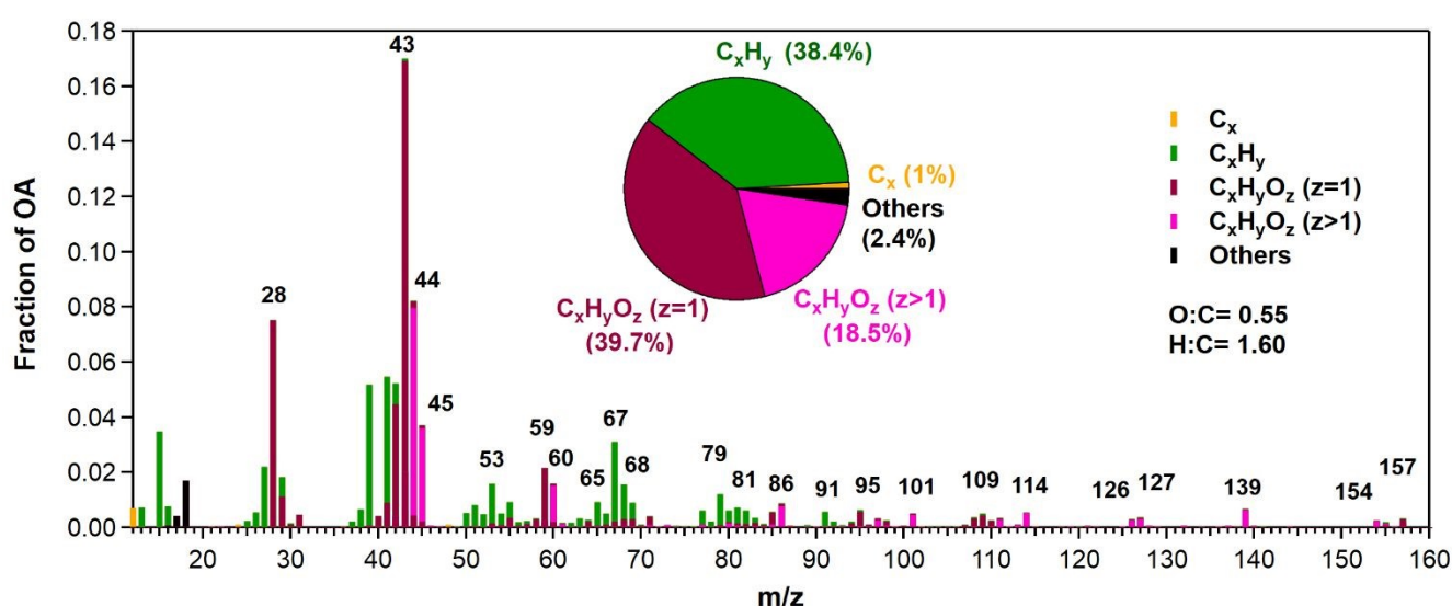
Figure 2. HR average AMS spectrum of pure diaterpenylic acid acetate (DTAA) aerosol. The most important characteristic m/z ratios were 53, 59, 60, 65, 67, 68, 69, 71, 77, 79, 80, 81, 82, 85, 86, 91, 95, 101, 109, 114, 126, 127, 139, 154 and 157.
