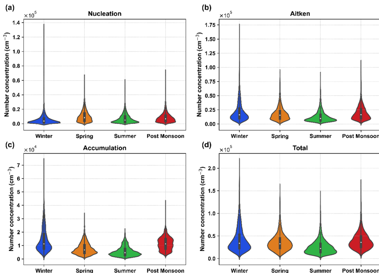
Fig. 1 Seasonal variation in average particle number concentrations of (a) nucleation mode, (b) Aitken mode, (c) accumulation mode, and (d) total, depicted using violin plots. These plots display the distribution and density of concentrations with the central white dot inside each box indicating the median value. The data reveal that total particle number concentration peaks during colder seasons (winter and post-monsoon), while the nucleation mode is more prevalent in warmer periods and the accumulation mode is more pronounced during colder periods.
