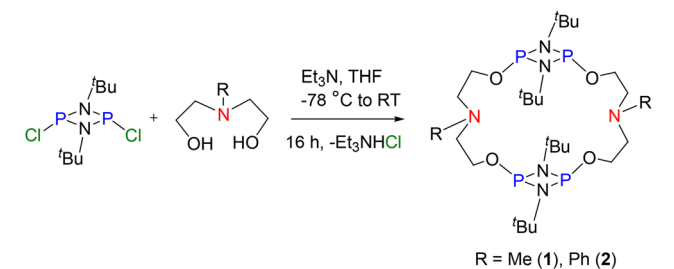
Scheme 1 Synthesis of macrocycles – [\{\text{P}(\mu\text{-N}^t\text{Bu})_2\}_2\{\text{O}(\text{CH}_2)_2\text{N}(\text{Me})(\text{CH}_2)_2\text{O}\}]_2 (1) and [\{\text{P}(\mu\text{-N}^t\text{Bu})_2\}_2\{\text{O}(\text{CH}_2)_2\text{N}(\text{Ph})(\text{CH}_2)_2\text{O}\}]_2 (2).
