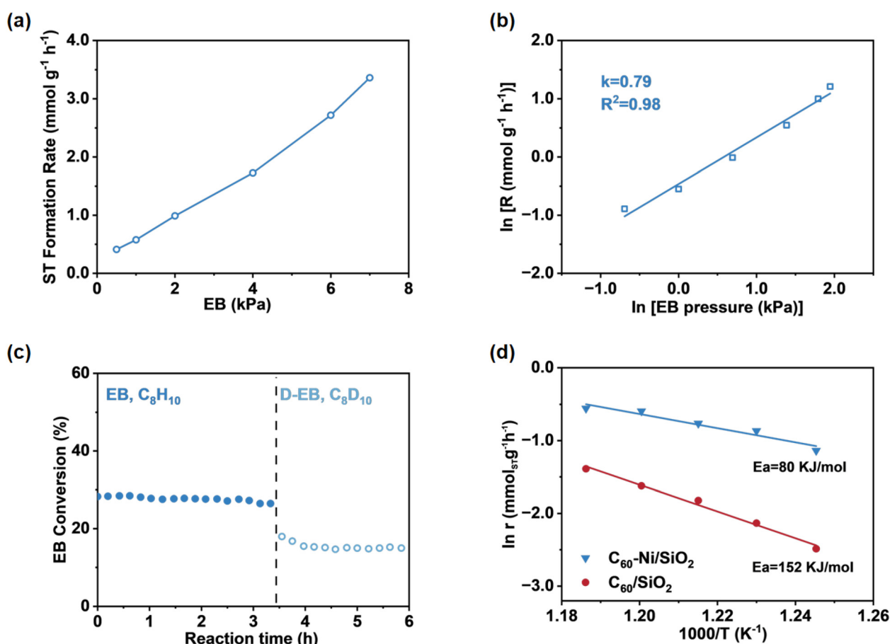
Fig. 4 (a) ST formation rates versus partial pressure of EB and (b) corresponding reaction order for the C_{60} -Ni/SiO 2 catalyst. Conditions: 100 mg catalyst, 550 °C, EB partial pressure 0.5–7.0 kPa, total flow 6.12 mL min −1 with He as balance gas, carbon balance: 100 ± 5%. (c) Time-on-stream EB conversion over the C_{60} -Ni/SiO 2 catalyst in EB ( C_8H_{10} )/He and D-EB ( C_8D_{10} )/He. Conditions: 100 mg catalyst, 550 °C, EB or D-EB partial pressure 1.0 kPa, total flow 6.12 mL min −1 with He as balance gas, carbon balance: 100 ± 5%. (d) Arrhenius plots for EB DDH over the C_{60} -Ni/SiO 2 and C_{60} /SiO 2 catalysts. Conditions: 100 mg catalyst, 530–570 °C, EB partial pressure 1.0 kPa, total flow 6.12 mL min −1 with He as balance gas, carbon balance: 100 ± 5%.
