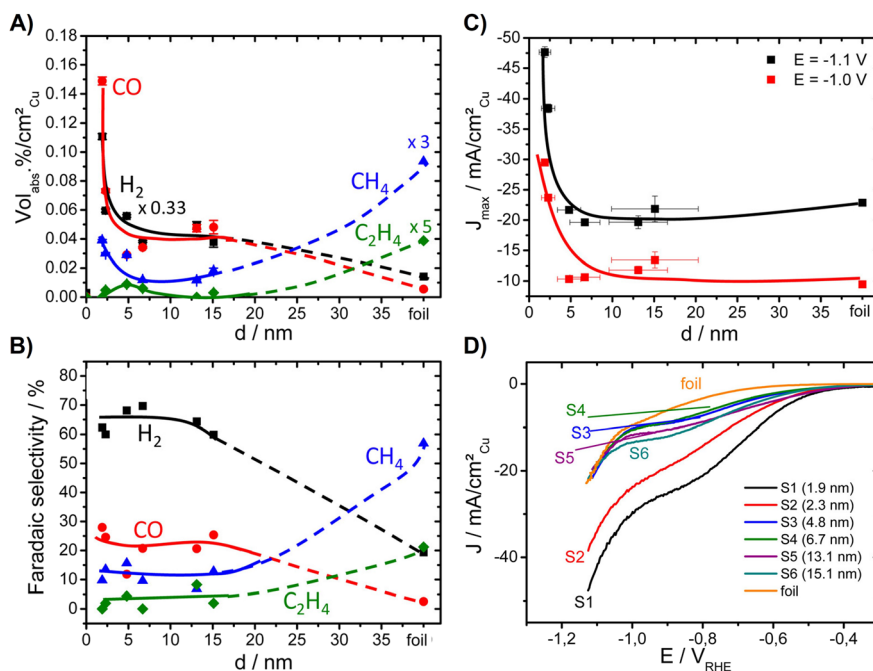
Fig. 29 Particle size dependence of (A) composition of gaseous reaction products (balance is CO 2 ) during catalytic CO 2 electroreduction over Cu NPs; (B) faradaic selectivity of reaction products during CO 2 electroreduction on Cu NPs; (C) particle size effect during catalytic CO 2 electroreduction, where the faradaic current densities at −1.1 and −1.0 V RHE −1 are plotted against the size of the Cu NP catalysts; and (D) linear sweep voltammetry of the CO 2 electroreduction on Cu NP catalysts, S1–S6, in 0.1 M KHCO 3 at room temperature and a scan rate of −5 mV s −1 . 307
