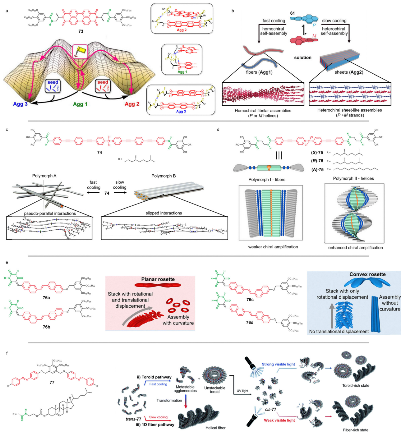
Fig. 20 (a) Molecular structure of compound 73 and the corresponding self-assembly energy landscape leading to the formation of Agg1 , Agg2 and Agg3 . The assembly mode of the three aggregates is schematically depicted in the inset (reproduced from ref. 339 with permission of the American Chemical Society, copyright 2019). (b) Scheme of the polymorphic behaviour of compound 61 forming fibres or sheet structures depending on the thermal treatment of the sample (reproduced from ref. 278 with permission of Wiley-VCH Verlag GmbH & Co. KGaA, Weinheim, copyright 2020). (c) Molecular structure of compound 74 and the scheme of its self-assembly behaviour forming polymorph A via pseudo-parallel interactions or polymorph B via slipped interactions depending on the thermal treatment of the sample (reproduced from ref. 340 with permission of American Chemical Society, copyright 2019). (d) Molecular structure of compounds (S)-75 , (R)-75 and (A)-75 and a schematic illustration of the corresponding polymorphs I and II providing distinct chiral amplification behaviour (reproduced from ref. 349 with permission of Wiley-VCH GmbH, copyright 2025). (e) Molecular structure of compounds 76a–d and a schematic illustration of the corresponding self-assembly behaviour into planar or convex rosettes and the subsequently into toroidal and fibrillar aggregates (reproduced from ref. 342 with permission of the Royal Society of Chemistry, copyright 2023). (f) Molecular structure of compound 77 and a scheme of its self-assembly behaviour including the light modulation of supramolecular polymorphism (reproduced from ref. 195 with permission of the Royal Society of Chemistry, copyright 2022).
