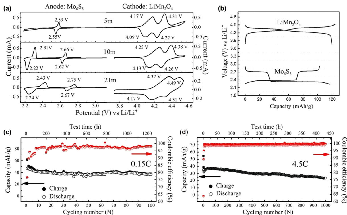
Fig. 6 (a) and (b) Cyclic voltammograms and galvanostatic charge and discharge curves of \text{LiMn}_2\text{O}_4 cathode and \text{Mo}_6\text{S}_8 anode in \text{LiTFSI}/\text{H}_2\text{O} with various concentrations. (c) and (d) Electrochemical performance of aqueous \text{LiMn}_2\text{O}_4|\text{Mo}_6\text{S}_8 full cells in water-in-salt 21 m \text{LiTFSI}/\text{H}_2\text{O} electrolyte. 18 Reprinted with permission from Science .
