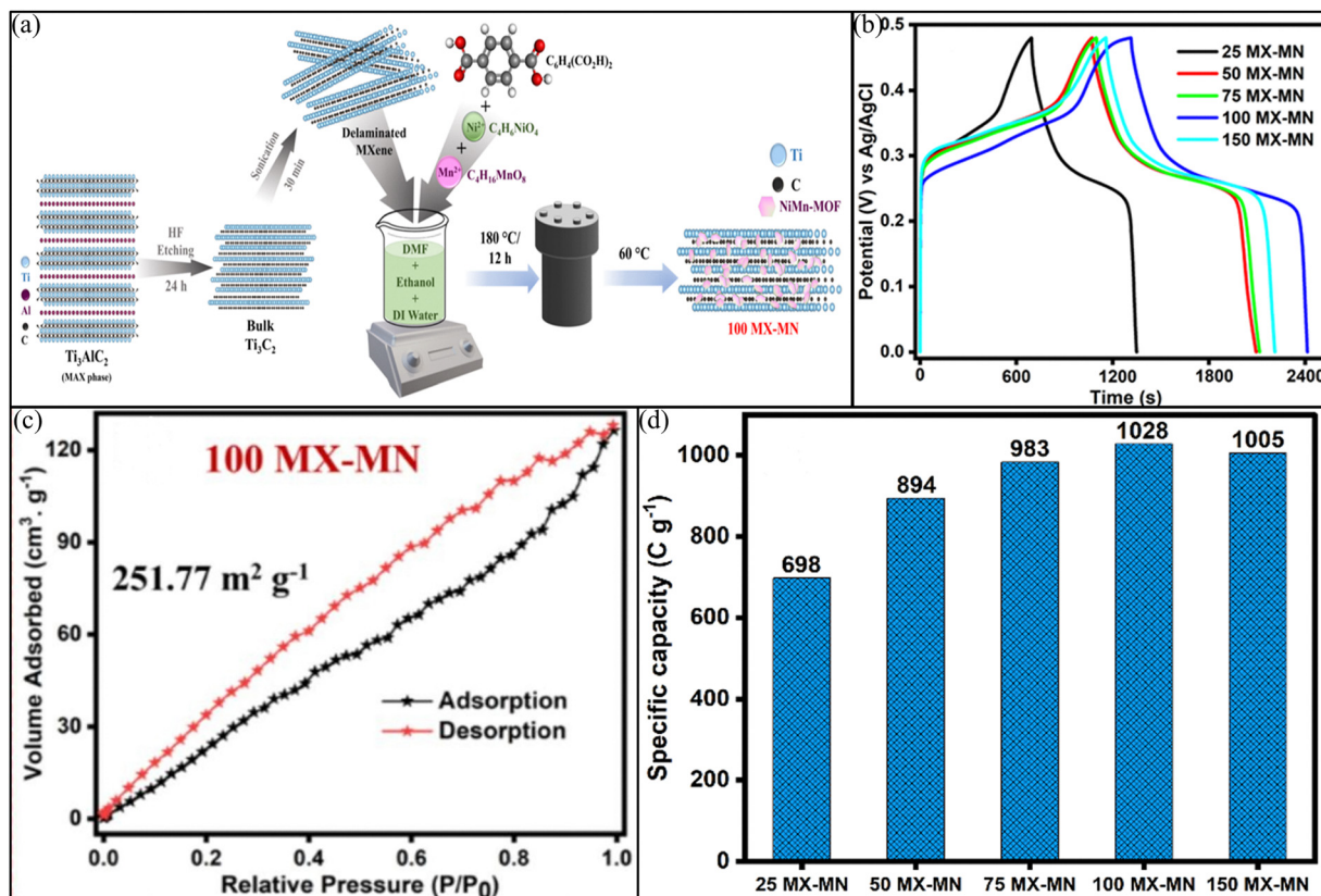
Fig. 19 (a) The schematic representation of etching aluminum from the MAX phase and the synthesis of composites. (b) The GCD curve at 1 \text{ A} \cdot \text{g}^{-1} , (c) the nitrogen adsorption–desorption and pore distribution curves of the 100 MX-MN composite, and (d) specific capacity of all the composites at 1 \text{ A} \cdot \text{g}^{-1} . Reproduced with permission from ref. 56. Copyright 2024, Elsevier.
