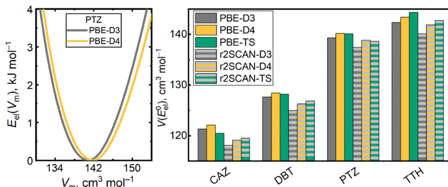
Fig. 3 Illustration of how static electronic energies E_{el} modelled by PBE-D3 and PBE-D4 for phenothiazine vary with respect to the molar volume V_m of the crystal (left); and a comparison of molar-volume coordinates V_0 of the minimum points of E_{el}(V_m) curves calculated for the target crystal forms using either PBE or r^2 SCAN functionals coupled with either D3, D4 or TS dispersion models (right).
