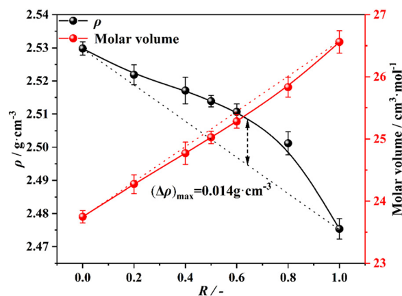
Fig. 5 Compositional dependence of the density ( \rho ) and molar volume of the 65.0\text{SiO}_2\text{-}5.0\text{B}_2\text{O}_3\text{-(}17.6 - x\text{)Na}_2\text{O-}x\text{K}_2\text{O-}7.5\text{CaO-}4.9\text{MgO} glasses as a function of different molar ratios R , where R is equal to the molar ratio of [\text{K}_2\text{O}]/([\text{Na}_2\text{O}] + [\text{K}_2\text{O}]) . The dashed line is a guide for the eye.
