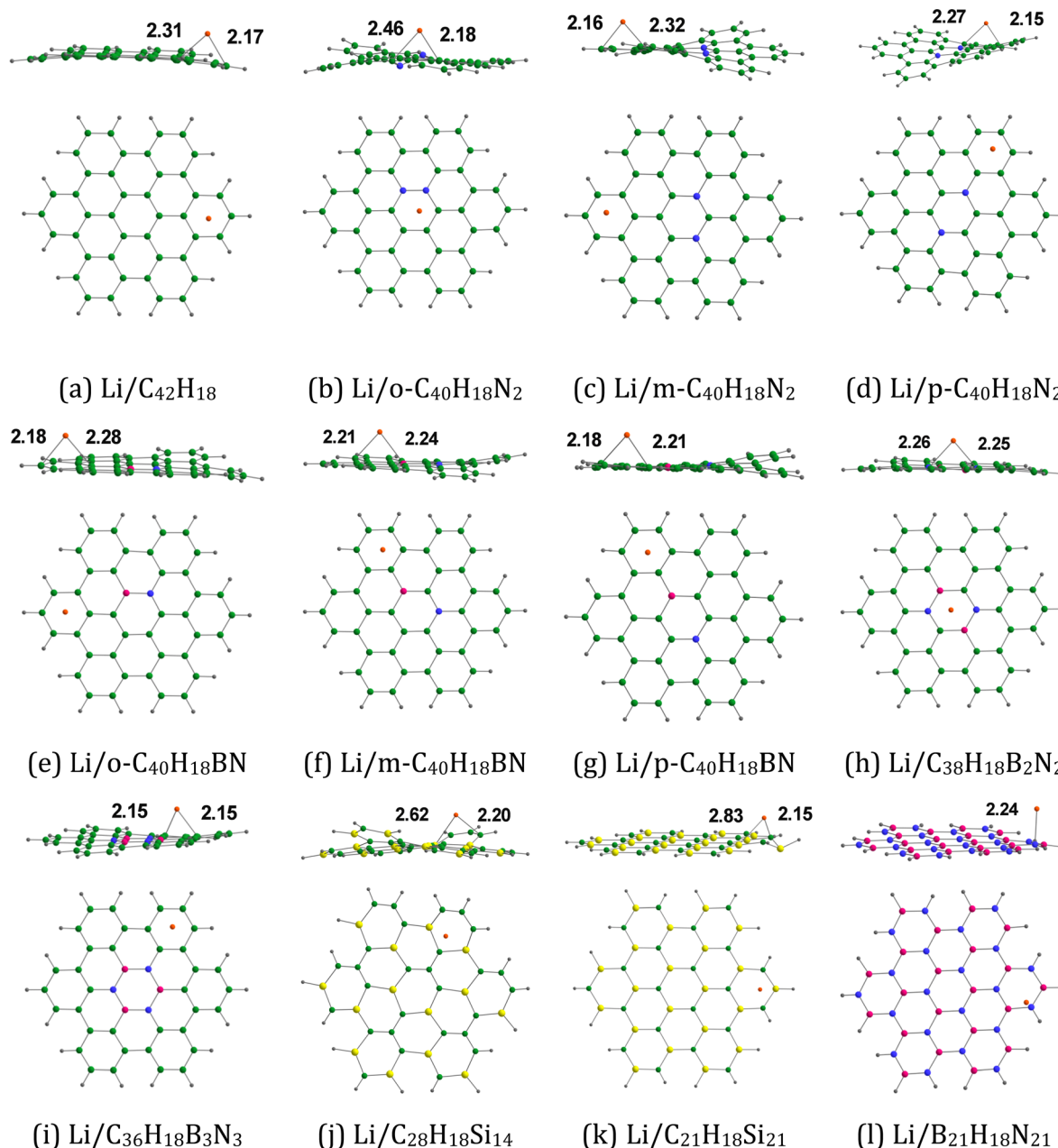
Fig. 6 Optimized structures of Li adsorbed on (a) C_{42}H_{18} , (b) o-C_{40}H_{18}N_2 , (c) m-C_{40}H_{18}N_2 , (d) p-C_{40}H_{18}N_2 , (e) o-C_{40}H_{18}BN , (f) m-C_{40}H_{18}BN , (g) p-C_{40}H_{18}BN , (h) C_{38}H_{18}B_2N_2 , (i) C_{36}H_{18}B_3N_3 , (j) C_{28}H_{18}Si_{14} , (k) C_{21}H_{18}Si_{21} , and (l) B_{21}H_{18}N_{21} . The bond distances are given in Å. The color code is the same as in Fig. 2. In addition, Li is denoted by the orange color.
