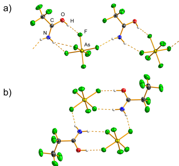
Fig. 2 Crystal structure of (a) the hydrogen-bonded chain in \text{CF}_3\text{C}(\text{OH})\text{NH}_2[\text{AsF}_6] and (b) the discrete hydrogen-bonded cluster in \text{C}_2\text{F}_5\text{C}(\text{OH})\text{NH}_2[\text{AsF}_6] (only one orientation of the disordered -\text{C}_2\text{F}_5 unit is shown). Hydrogen bonds are shown as dashed orange lines. Displacement ellipsoids are drawn at the 50% probability level, and hydrogen atoms are represented as spheres of arbitrary radius.
