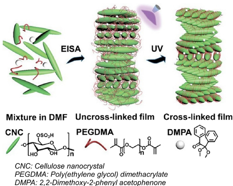
Fig. 13 A simple and robust method to co-assemble cellulose nanocrystals with poly(ethylene glycol)dimethacrylate (PEGDMA) monomers in N,N -dimethylformamide by integration of cellulose nanocrystal self-assembly with UV-initiated polymerisation. Reprinted with permission from ref. 57 copyright 2022 Wiley-VCH.
