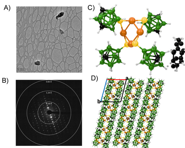
Fig. 2 MicroED reveals solvent inclusion in the \text{Cu}_4(m_9\text{-CBT})_4 structure. (A) TEM image of microcrystals. (B) Initial diffraction frames showing high-resolution data. (C) Resolved structure highlighting the disordered toluene molecule undetectable by SC-XRD. (D) 3 \times 3 \times 3 crystal packing along c -axis. Color code: Cu (orange), S (yellow), B (green), C (black), H (white).
