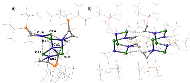
Fig. 2 Solid-state structure of ( 1 ). (a) The Cu 4 Cl 4 -core and SiCCH drawn as thermal ellipsoids (50% probability levels); i Pr-groups are rendered as wire frame for clarity. (b) Weak hydrogen bonding (CC-H...Cl) linking clusters of 1 into a 1D-network.
