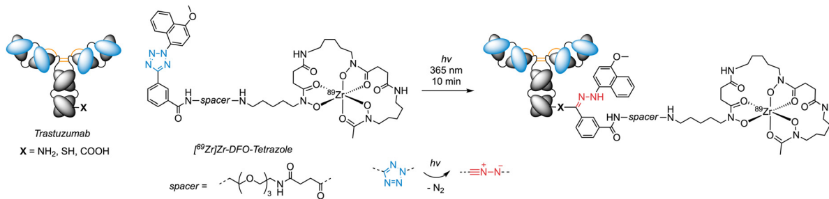
Scheme 4 Photo(radio)synthesis of functionalised proteins using light-induced activation of tetrazoles. Formation of the electronic excited state of a tetrazole can lead to intramolecular rearrangements and loss of N_2(g) to generate a 1,3-dipolar nitrile imine. This intermediate finds applications in labelling compounds bearing alkene or alkyne reaction partners (photo-click) or in direct reaction with biologically relevant nucleophiles found on protein.
