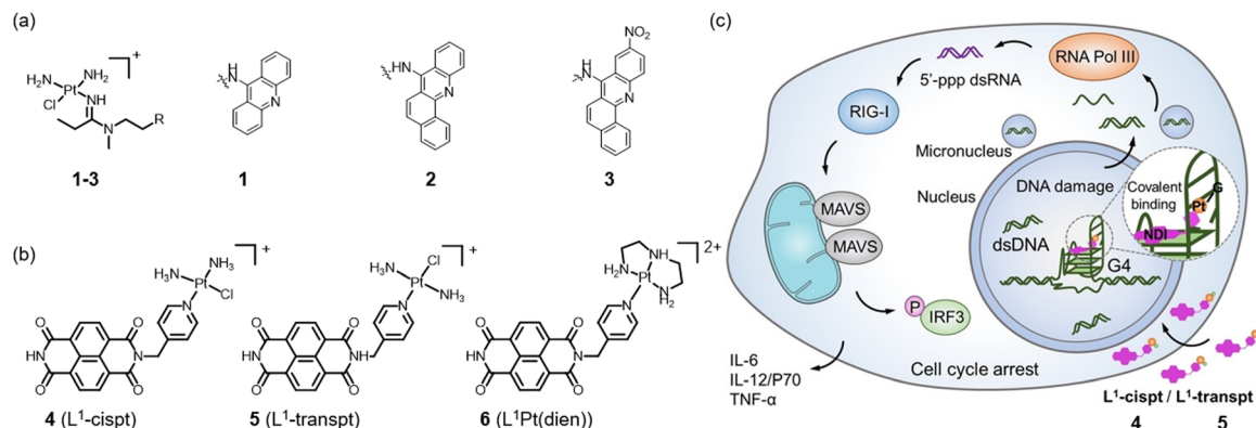
Fig. 2 (a) and (b) The chemical structures of representative mono-chelated platinum complexes 1–6 reported in the literature. (c) The G-quadruplex-binding platinum complexes 4 and 5 can damage DNA, increase micronucleus formation, activate the RIG-I pathway, and induce ICD in vivo . 39 Copyright©2023, John Wiley and Sons.
