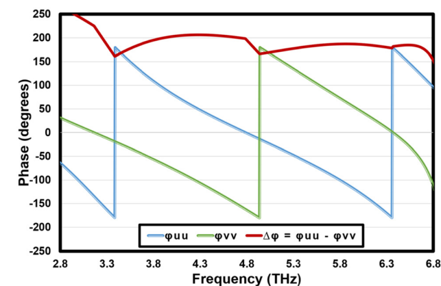
Fig. 9 Phase difference between \phi_{uu} and \phi_{vv} demonstrating near 180° shift required for effective polarization conversion.
