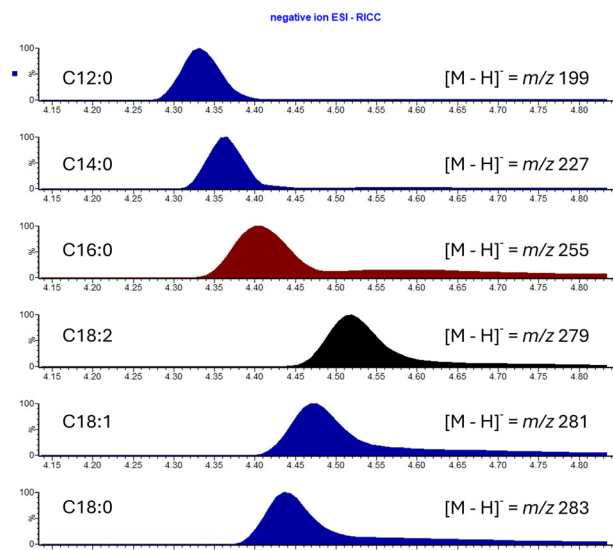
Fig. 5 Reconstructed ion current chromatogram (RICC) of the negative ion ESI SFC-MS of HVO 3.
