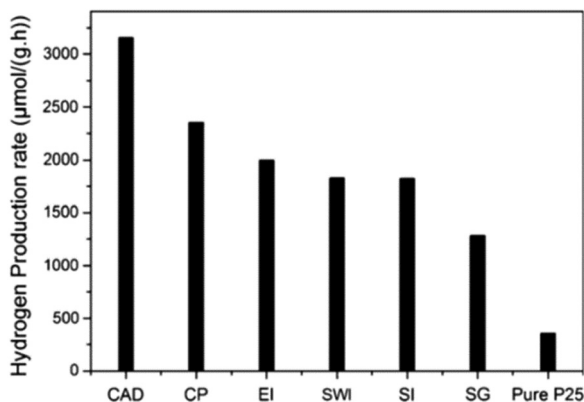
Fig. 17 Comparison of the photocatalytic hydrogen evolution rate on pure P25 and \text{CuO}/\text{TiO}_2 samples produced by different preparation methods, namely chemical adsorption decomposition (CAD), composite precipitation (CP), ethanol impregnation (EI), simple wet impregnation (SWI), stepwise impregnation (SI), and sol-gel (SG). Reproduced with permission from ref. 184. Copyright © 2014, Springer.
