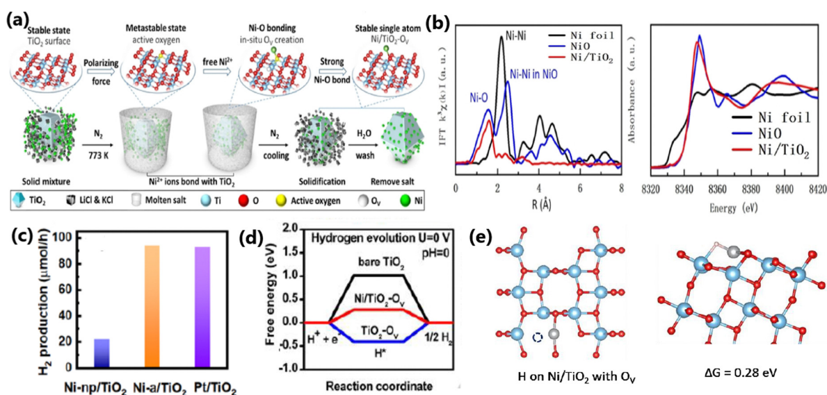
Fig. 18 (a) Schematic illustration of molten salt-mediated preparation of atomic Ni on \text{TiO}_2 . For the \text{TiO}_2 molecular structure, (b) EXAFS and XANES spectra of \text{Ni}/\text{TiO}_2 , respectively. Ni loading amount: 0.46 wt% (c) Comparison of \text{H}_2 evolution activity on \text{Ni-np}/\text{TiO}_2 , \text{Ni-a}/\text{TiO}_2 and \text{Pt}/\text{TiO}_2 with the same loading amount ( \sim 0.5 \text{ wt\%} ). Experimental condition: 50 mg of sample dispersed in 100 mL of 10 vol% methanol aqueous solution (278 K) under an irradiation of a 300 W Xe lamp. (d) Free energy versus the reaction coordinates of different active sites. The simulation is based on the (101) facet of anatase \text{TiO}_2 . (e) Molecular models of \text{O}_v on \text{Ni}/\text{TiO}_2 and the corresponding formation energy of \text{O}_v . Reproduced with permission from ref. 172. Copyright © 2020, Wiley-VCH.
