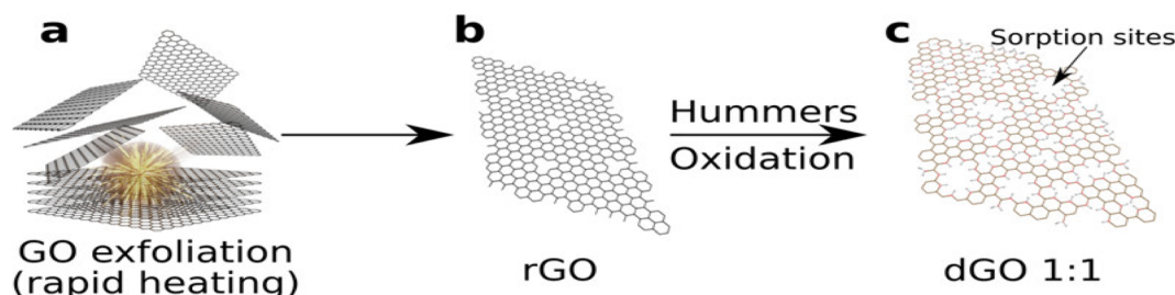
Fig. 7 Scheme for the preparation of defective GO: (a) explosive thermal-exfoliation of GO, (b) Hummer's oxidation of defective rGO and (c) dGO with sorption sites. 219
