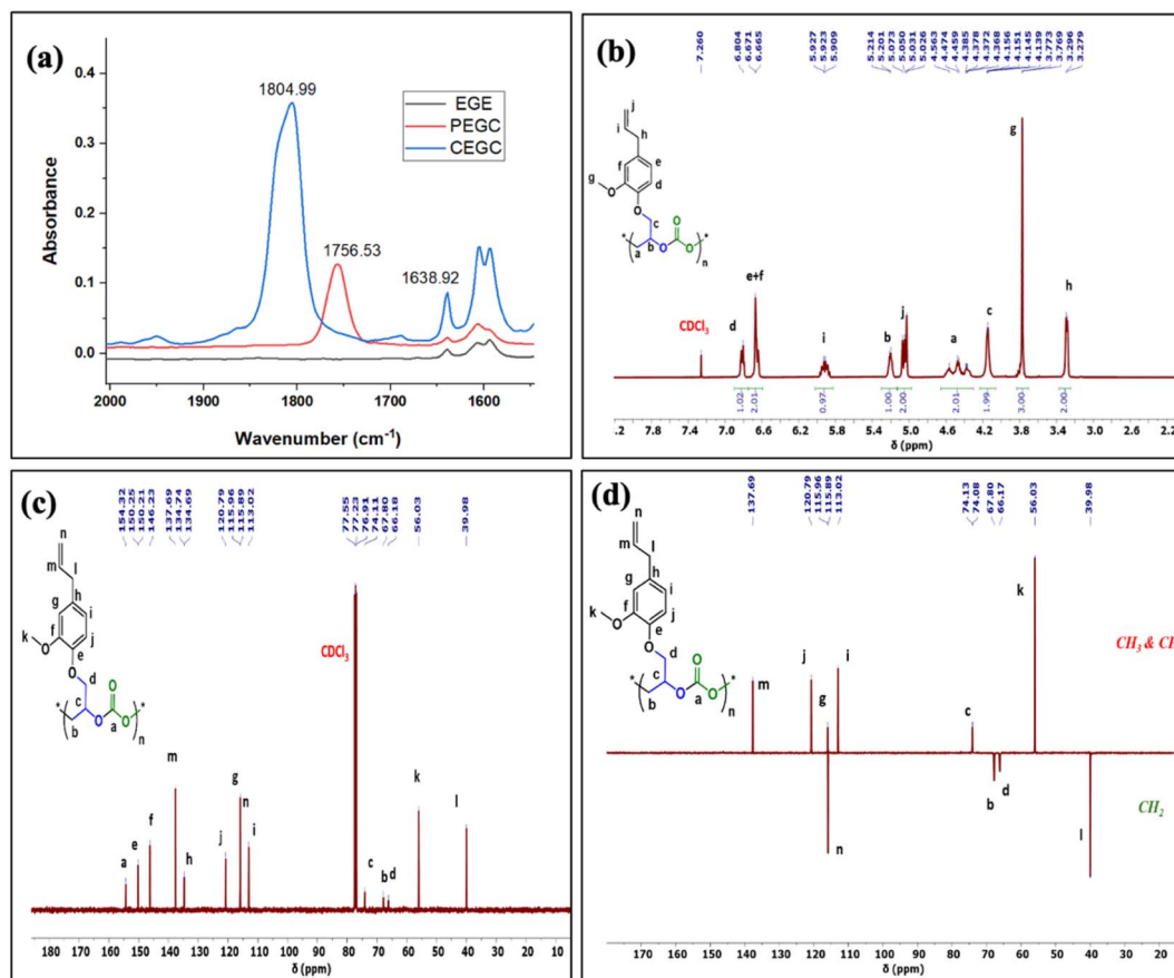
Fig. 5 (a) Comparison of ATR FT-IR spectrum of EGE, cyclic carbonate (CEGC), and polycarbonate (PEGC) in \text{CH}_2\text{Cl}_2 . (b) ^1\text{H} - and (c) ^{13}\text{C} -NMR and (d) ^{13}\text{C} (DEPT-135) spectra of polycarbonate polymers of EGE/ \text{CO}_2 in \text{CDCl}_3 .
