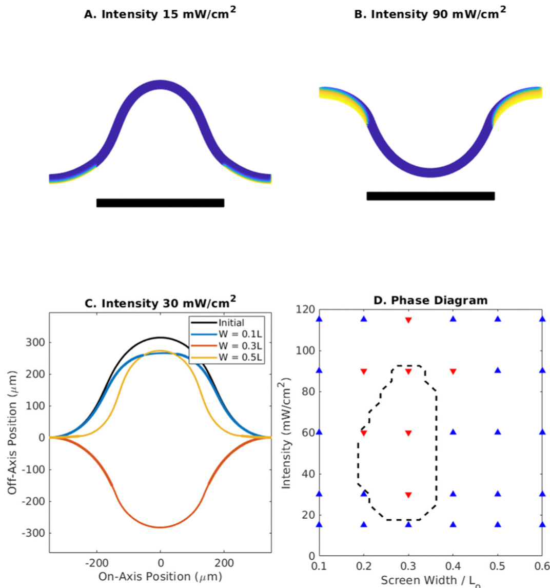
Fig. 7 Snap-through in opposite direction (A) final conformation from finite element simulation with intensity 15 mW cm -2 and screen width 400 μm. The strip remains in the upward-buckled state. (B) Final conformation at higher intensity (90 mW cm -2 ). The curvature induced by the bimorph at the edges causes the strip to snap through towards the light. (C) Effect of screen width variation at constant intensity 30 mW cm -2 . The initial conformation is indicated via the black line. For a narrow screen (100 μm, blue line), the energy difference between buckled states is insufficient to induce snap-through. For a wider screen (300 μm, orange line) the strip can reduce free energy by snapping through to the downward-buckled conformation. When a 500 μm region is blocked (yellow line) the system is stable in its original state. (D) Phase diagram showing the values of screen width and intensity for which finite element simulations initially buckled away from the light underwent snap-through towards the light (red) or remained in initial state (blue). Black dashed line indicates phase boundary predicted by semi-analytical model. As with the centered aperture, there is a range of intensities and widths bounded above and below for which snapthrough occurs.
