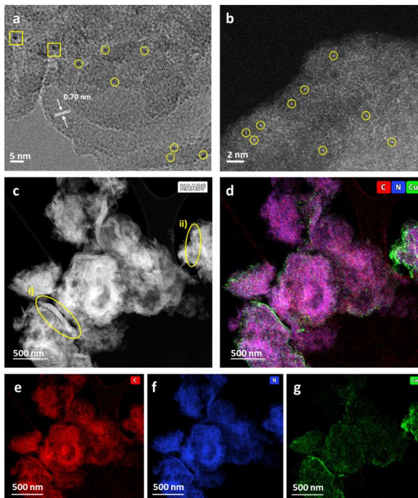
Fig. 4 (a) HRTEM image at 200 kV of Cu/nc-C 3 N 4 with a spacing of 0.7 nm between tri-s-triazine units, showing Cu atoms (yellow circles) and CuNPs (yellow squares). (b) AC-STEM image showing Cu atoms (yellow circles). (c) HAADF-STEM image of Cu/nc-C 3 N 4 , nanocrystalline domains pertain to brighter areas of the image and the remainder to amorphous carbon nitride domains. Measurable nanocrystalline domains are encircled (yellow). (d) Composed STEM-EDX map of all components overlapping: C (red), N (blue), Cu (green). (e), (f) and (g) Single elemental maps of C, N and Cu respectively.
