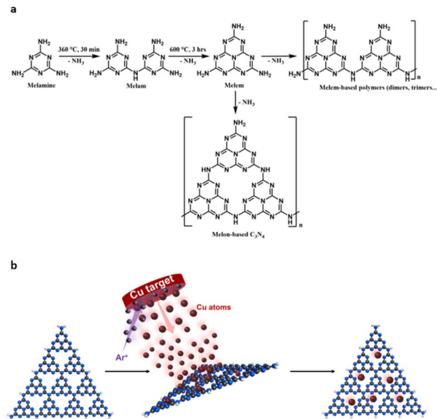
Fig. 7 (a) Synthesis of \text{b-C}_3\text{N}_4 from melamine via a two-step calcination method. Polycondensation under these conditions can yield melon- and/or melon-based polymers. (b) Schematic representation of Cu atoms deposition by sputtering metal atoms from the solid metal target in vacuum directly onto carbon nitride (copper red, carbon grey, nitrogen blue, hydrogen white).
