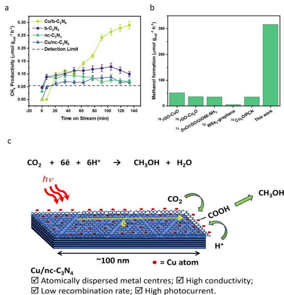
Fig. 6 Catalyst performance in photocatalytic reduction of \text{CO}_2 . (a) \text{CH}_4 productivity over time ( \mu\text{mol g}_{\text{cat}}^{-1} \text{h}^{-1} ) for \text{Cu/b-C}_3\text{N}_4 (light green circle), \text{Cu/nc-C}_3\text{N}_4 (blue triangle), \text{b-C}_3\text{N}_4 (purple circle) and \text{nc-C}_3\text{N}_4 (green triangle). (b) Literature comparison of methanol formation rate ( \mu\text{mol g}_{\text{cat}}^{-1} \text{h}^{-1} ) produced over other visible light active catalysts and \text{Cu/nc-C}_3\text{N}_4 (this work) catalyst (Fig. S11†). 67–71 (c) Schematic representation of \text{CO}_2 photoreduction on a nanocrystalline domain of carbon nitride decorated with single copper atoms.
