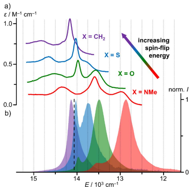
Fig. 3 (a) NIR absorption spectra and (b) normalised emission spectra of [1^{\text{X}}]^{3+} ( \text{X} = \text{CH}_2 , \lambda_{\text{exc}} = 460 \text{ nm} ), [1^{\text{S}}]^{3+} (blue, \lambda_{\text{exc}} = 450 \text{ nm} ), [1^{\text{O}}]^{3+} (green, \lambda_{\text{exc}} = 450 \text{ nm} ) and [1^{\text{NMe}}]^{3+} (red, \lambda_{\text{exc}} = 435 \text{ nm} ) in \text{CH}_3\text{CN} at room temperature. For clarity, the absorption spectra of [1^{\text{X}}]^{3+} with \text{X} = \text{O} , \text{S} , \text{CH}_2 were shifted vertically by +0.2 , +0.4 and +0.6 \text{ M}^{-1} \text{ cm}^{-1} . The dashed black line marks the energy of the 4th pyridine CH overtone \tilde{\nu}_{\text{CH}_4} . 25
