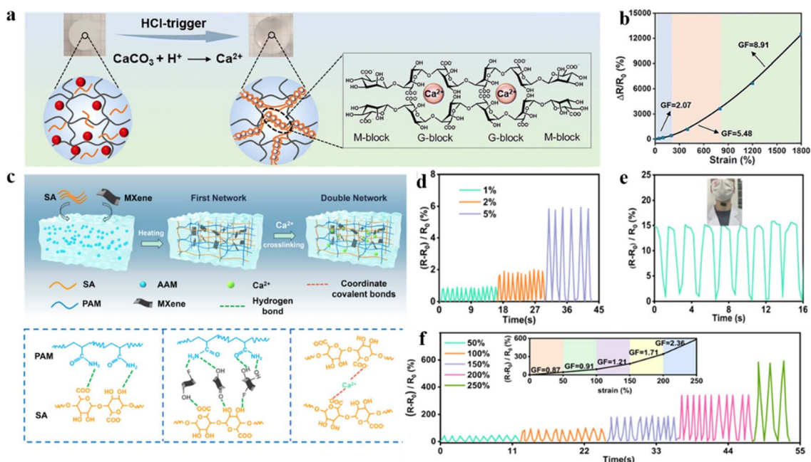
Fig. 13 Metal ion modification strategies under extreme mechanical strength conditions. (a) Schematic diagram of acid-triggered Ca 2+ release and SA network cross-linking. (b) Relative resistance changes to tensile strain in Ca 2+ /SA/PAM-DN hydrogels. Reproduced from ref. 162. Copyright 2023, Royal Society of Chemistry. (c) Schematic illustration of the fabrication of the PSM-DN hydrogels. (d) Relative resistance change of the PSM-Ca 2+ hydrogel based on minor strain. (e) Resistance changes of the PSM-Ca 2+ hydrogel strain sensor for swallowing movements. (f) Relative resistance change of the PSM-Ca 2+ hydrogel based on large strain and GF. Reproduced from ref. 163. Copyright 2023, The American Chemical Society.
